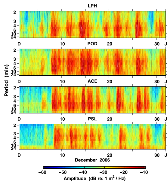
Figure 2. Spectral levels of 1-min tide gauge data in the infragravity-wave band along the U.S. west coast from northern Washington (LPH) to southern California (PSL; see Figure 3a for locations). The typical slight shift in energy to later times results from the lag associated with southward propagation of the IG wave-generating swell along the coast (Figure 1e). No time shift between stations implies IG wave generation from ocean waves at nearly the same time over a long stretch of coastline. The tide gauge data are collected with an acoustic water level sensor having a 3 m dynamic range over 1 s with a 0.1 mm resolution, and averaged to 1 min. The mode 1 principal component of these data is shown in Figure 3b.
