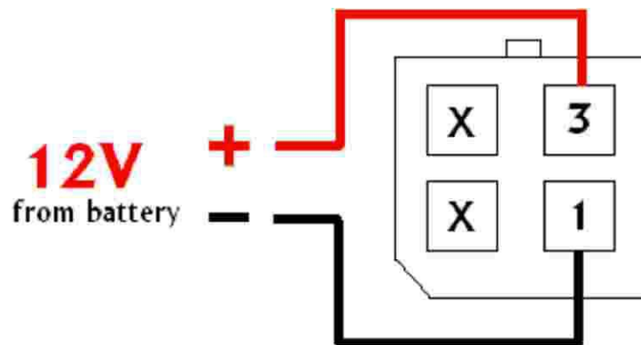
Molex Minifit 4 Pos. Male (FACE VIEW)
