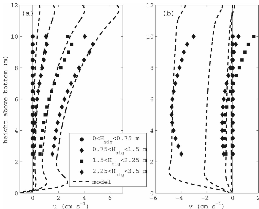
FIG. 11. Average (a) cross-shelf u and (b) along-shelf v velocity profiles from MVCO for different ranges of H_{sig} during periods when the wind stress magnitude was small ( |\tau^*| < 0.03 \text{ N m}^{-2} ) and corresponding model profiles (dashed lines) estimated using the average wave characteristics for each range of H_{sig} and a constant eddy viscosity A = 10^{-5} \text{ m}^2 \text{ s}^{-1} . Observed profiles for H_{sig} < 0.75 \text{ m} are zero because the weak wind and small wave mean profile (Fig. 10) has been subtracted from all profiles. Standard errors of the means for the observed profiles are 0.1 \text{ cm s}^{-1} for 0 < H_{sig} < 0.75 \text{ m} , 0.4 \text{ cm s}^{-1} for 0.75 < H_{sig} < 1.5 \text{ m} , 0.4 \text{ cm s}^{-1} for 1.5 < H_{sig} < 2.25 \text{ m} , and 1.6 \text{ cm s}^{-1} for 2.25 < H_{sig} < 3.5 \text{ m} . The reduced offshore currents in the top bin (height 10 m) may be due to contamination by surface reflections from the sidelobes of the ADCP acoustic pulses during large waves because of the reduced water depth under the wave troughs.
