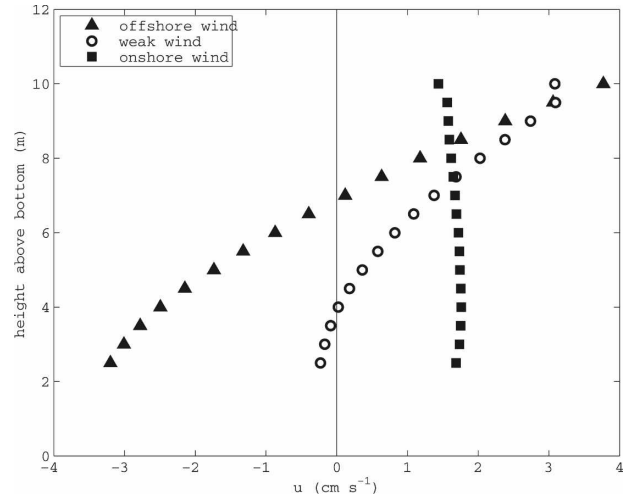
FIG. 9. Average offshore flow profiles from MVCO for periods when 1 \text{ m} < H_{\text{sig}} < 2 \text{ m} , and the wind stress was either offshore ( 0.1 \text{ N m}^{-2} < \tau^{sx} < 0.2 \text{ N m}^{-2} ), onshore ( -0.2 \text{ N m}^{-2} < \tau^{sx} < -0.1 \text{ N m}^{-2} ), or weak ( |\tau^s| < 0.03 \text{ N m}^{-2} ).
