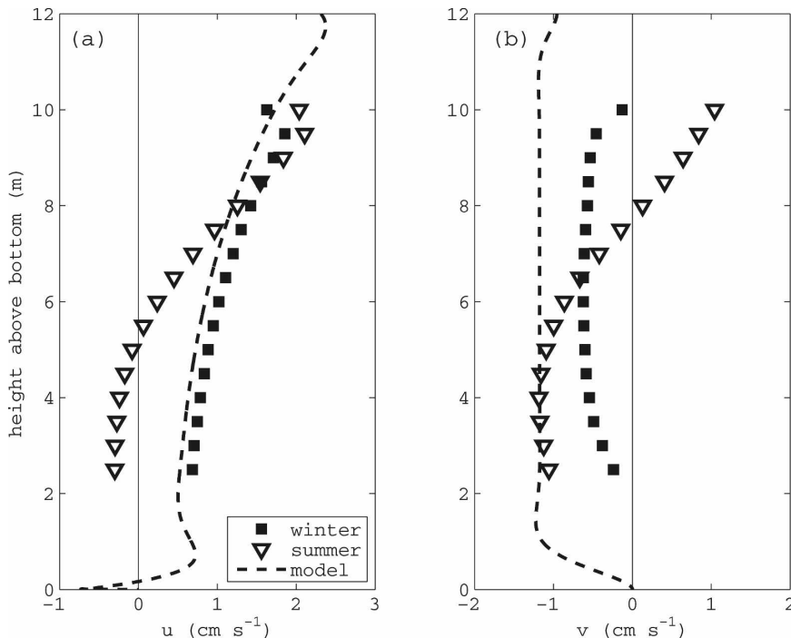
FIG. 12. Average (a) cross-shelf u and (b) along-shelf v velocity profiles from MVCO for 1 \text{ m} < H_{\text{sig}} < 2 \text{ m} and |\tau^{\text{sy}}| < 0.03 \text{ N m}^{-2} during winter (October–March) and summer (April–September) and from the model for A = 10^{-5} \text{ m}^2 \text{ s}^{-1} using the average wave characteristics for the selected observations. Only the average model profile is shown because the summer and winter model profiles are similar and the average wave characteristics are essentially the same. Standard errors of the means are 0.3 \text{ cm s}^{-1} for the winter profile and 0.5 \text{ cm s}^{-1} for the summer profile.
