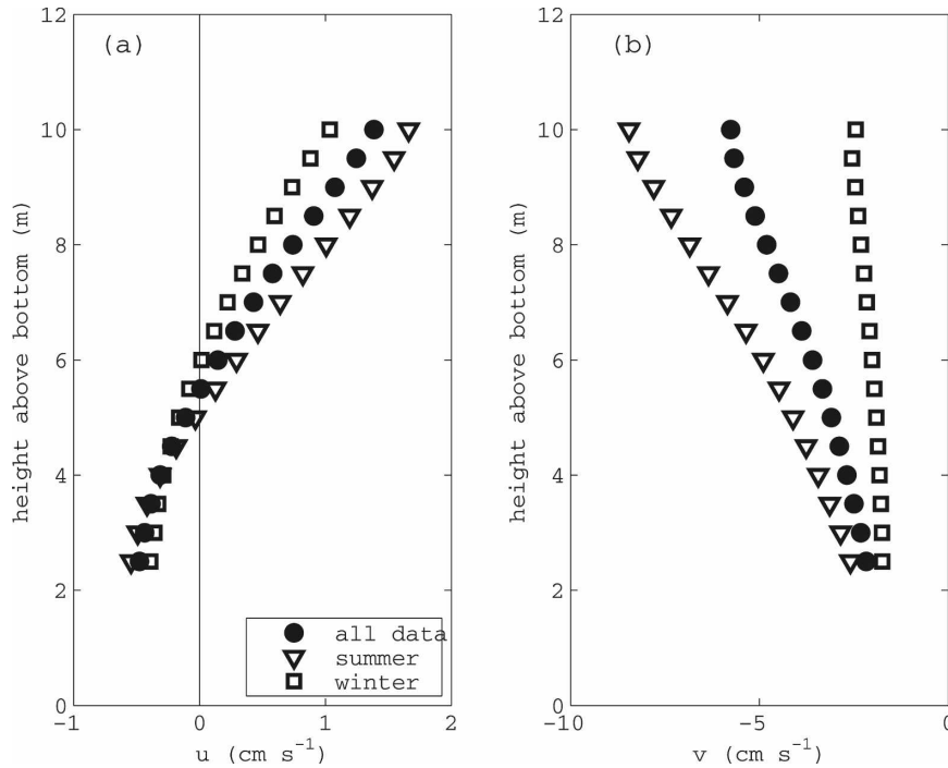
FIG. 10. Average (a) cross-shelf u and (b) along-shelf v velocity profiles from MVCO for periods when the waves are small ( H_{sig} < 0.75 m) and the wind stress is weak ( |\tau^s| < 0.03 N m -2 ) for all data, summer (April–September), and winter (October–March).
